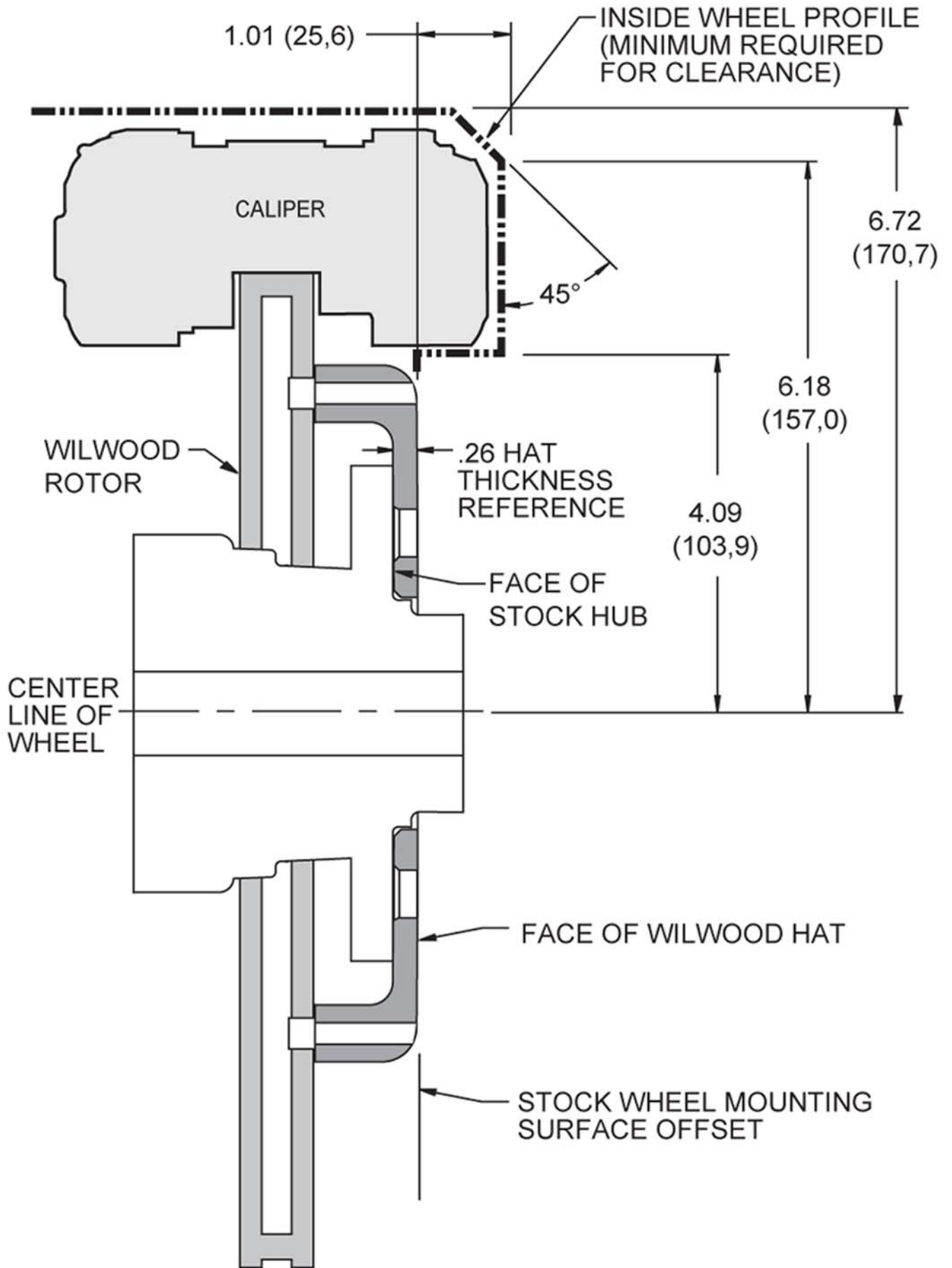
Wheel Clearance Diagram - 11.75" Rotor
